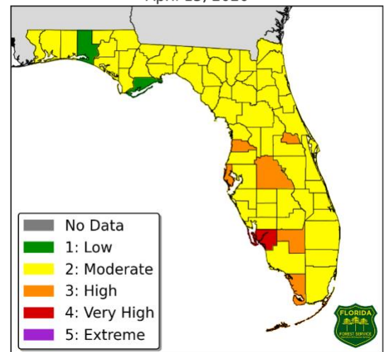
Forecast Fire Danger Indices April 13, 2020
