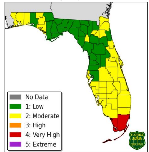
Forecast Fire Danger Indices April 24, 2020
