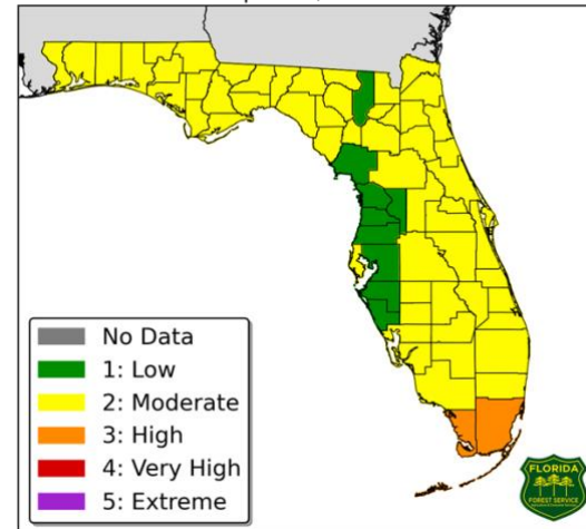
Forecast Fire Danger Indices April 30, 2020
