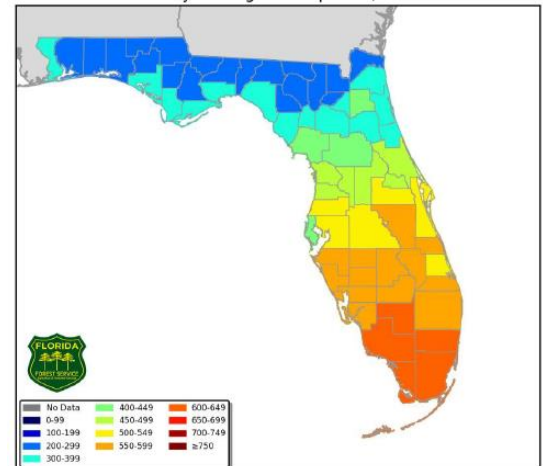
Keetch Byram Drought Index (KBDI) County Averages for April 04, 2020
