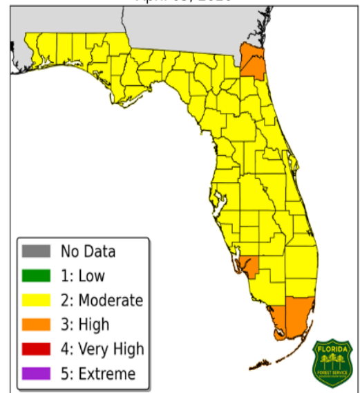
Forecast Fire Danger Indices April 09, 2020
